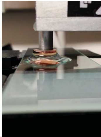
Figure B.5: Actual representation of the stem from the contact mechanics test in which the equilibrating procedure of the hemispherical hydrogel adhesive with 250\mu\text{m} of the pH 9 buffer solution
