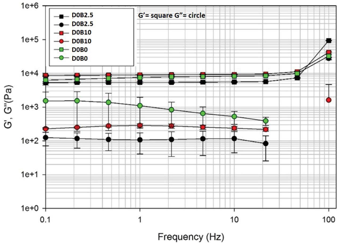
Figure B.11: Comparing the storage and loss moduli for increasing amounts of AAPBA at pH 9
