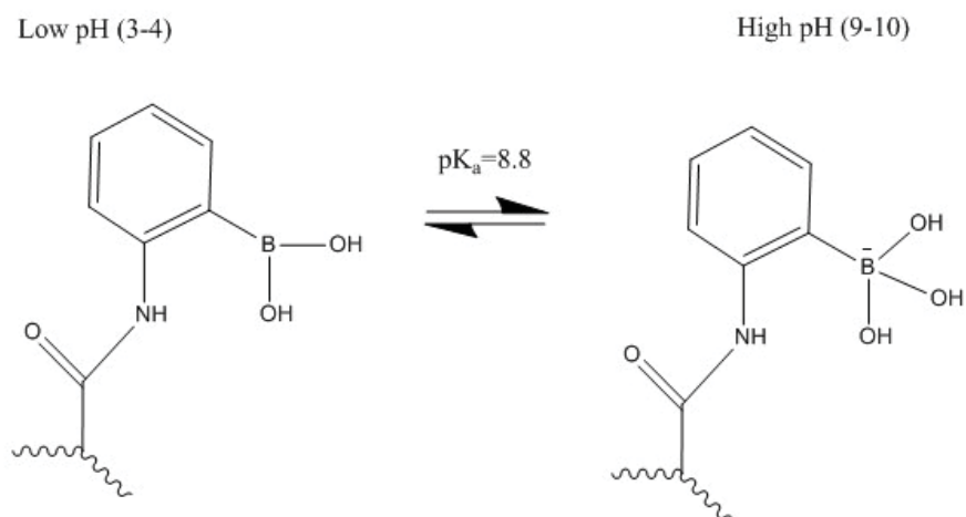
Figure 4.4: Figure showing the tetrahedral moiety of AAPBA at pH values above the pK_a of PBA
